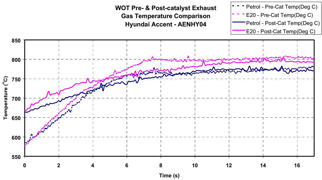
Figure 5.8 - WOT Exhaust Temperatures Hyundai Accent - AENHY04
