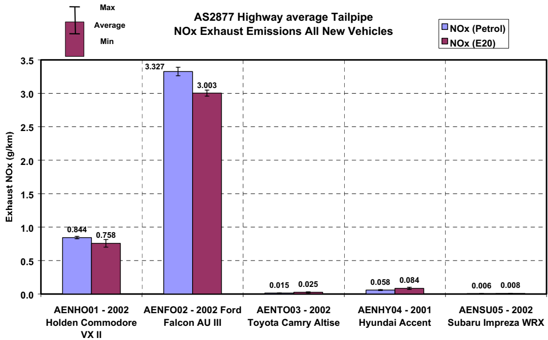
Figure 5.21 - AS2877 Highway Tailpipe NOx Emissions All New Vehicles
