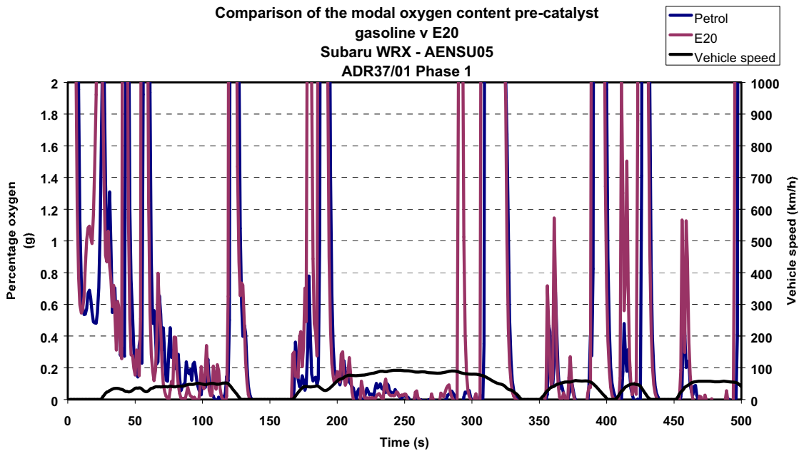
Figure 5.40 - Comparison of the Percentage Oxygen Content Pre-Catalyst Gasoline vs. E20 Subaru WRX (AENSU05)
