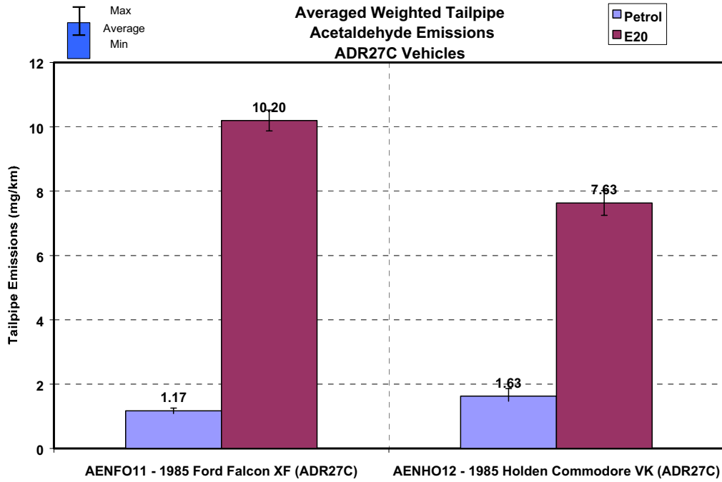
Figure 5.117 - ADR27C Average Weighted Tailpipe Acetaldehyde Emissions
