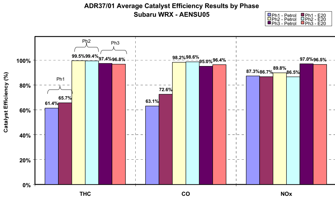
Figure 5.46 - Average Catalyst Efficiency Subaru WRX AENSU05
