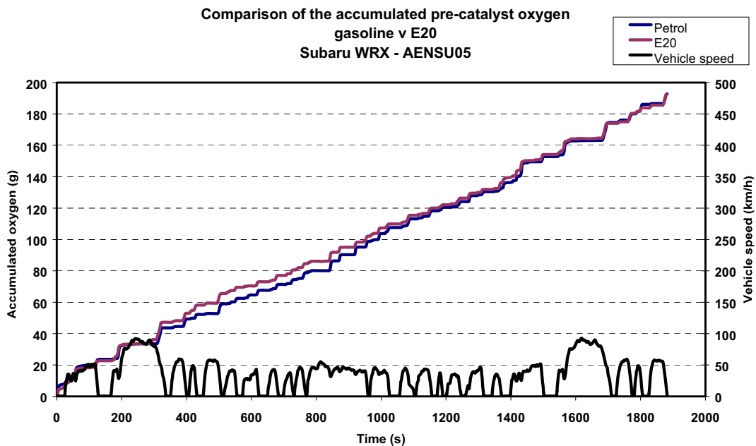
Figure 5.41 - Comparison of the Accumulated Pre-Catalyst Oxygen Gasoline vs. E20 Subaru WRX (AENSU05).
