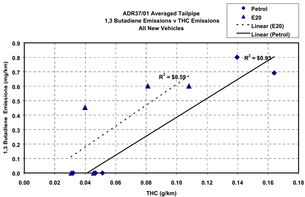
Figure 5.62 Relationship Between 1,3 Butadiene and THC Tailpipe Emissions.
