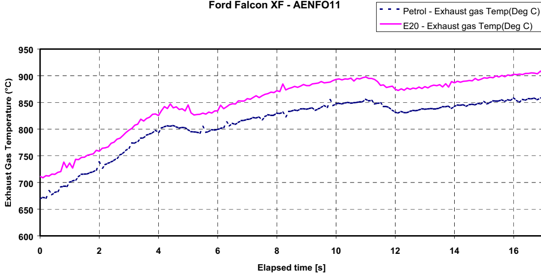
Comparison of Exhaust Gas Temperature for Standing start Ford Falcon XF - AENFO11
