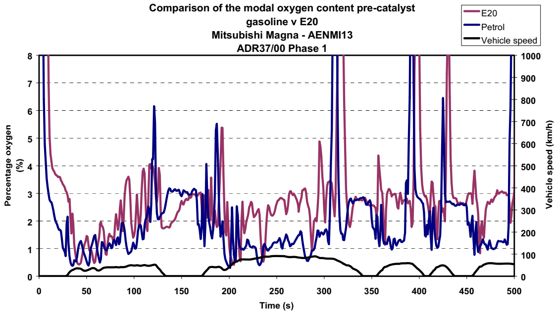
Figure 5.107 - Comparison of the Percentage Oxygen Content Pre-Catalyst Gasoline vs. E20 Mitsubishi Magna (AENMI13).
