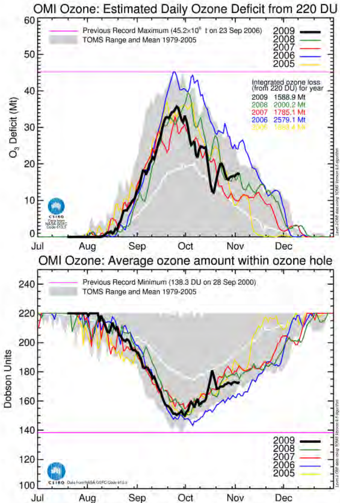
Figure 2: Estimated daily ozone deficit (top panel) and average ozone amount within the ozone hole (bottom panel) based on OMI satellite data, as of 3 November 2009.
