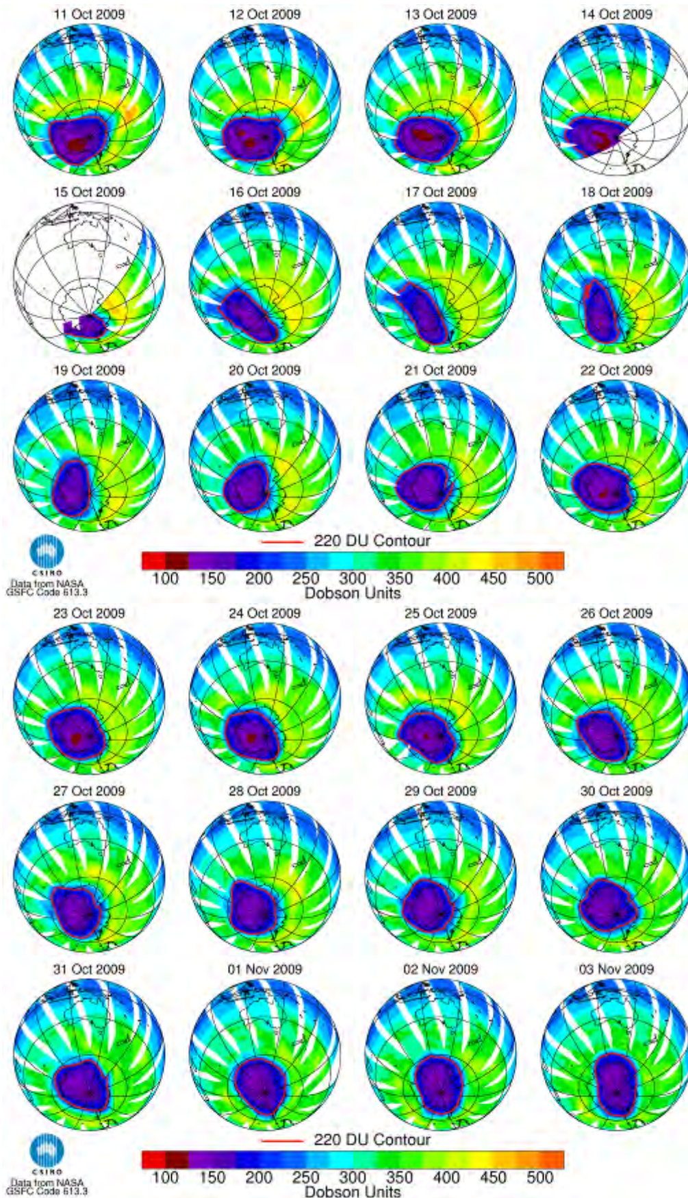
Figure 3: OMI ozone hole images for 11 October to 3 November 2009; the ozone hole boundary is indicated by the red 220 DU contour line. The white stripes are bad/missing data due to a physical obstruction in the OMI instrument field of view.
