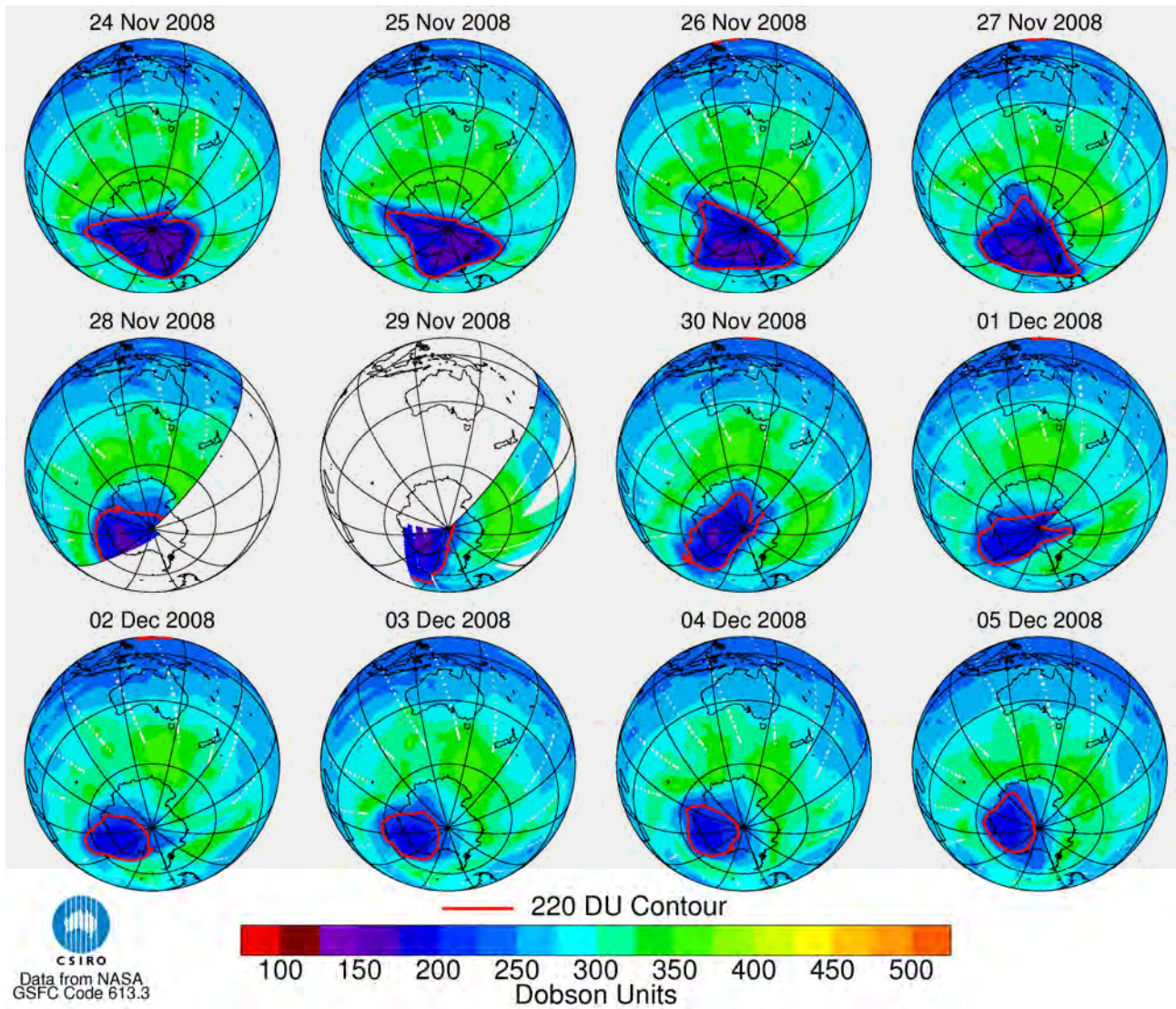
Figure 3: OMI ozone hole images for 24 November to 5 December 2008; the ozone hole boundary is indicated by the red 220 DU contour line.
