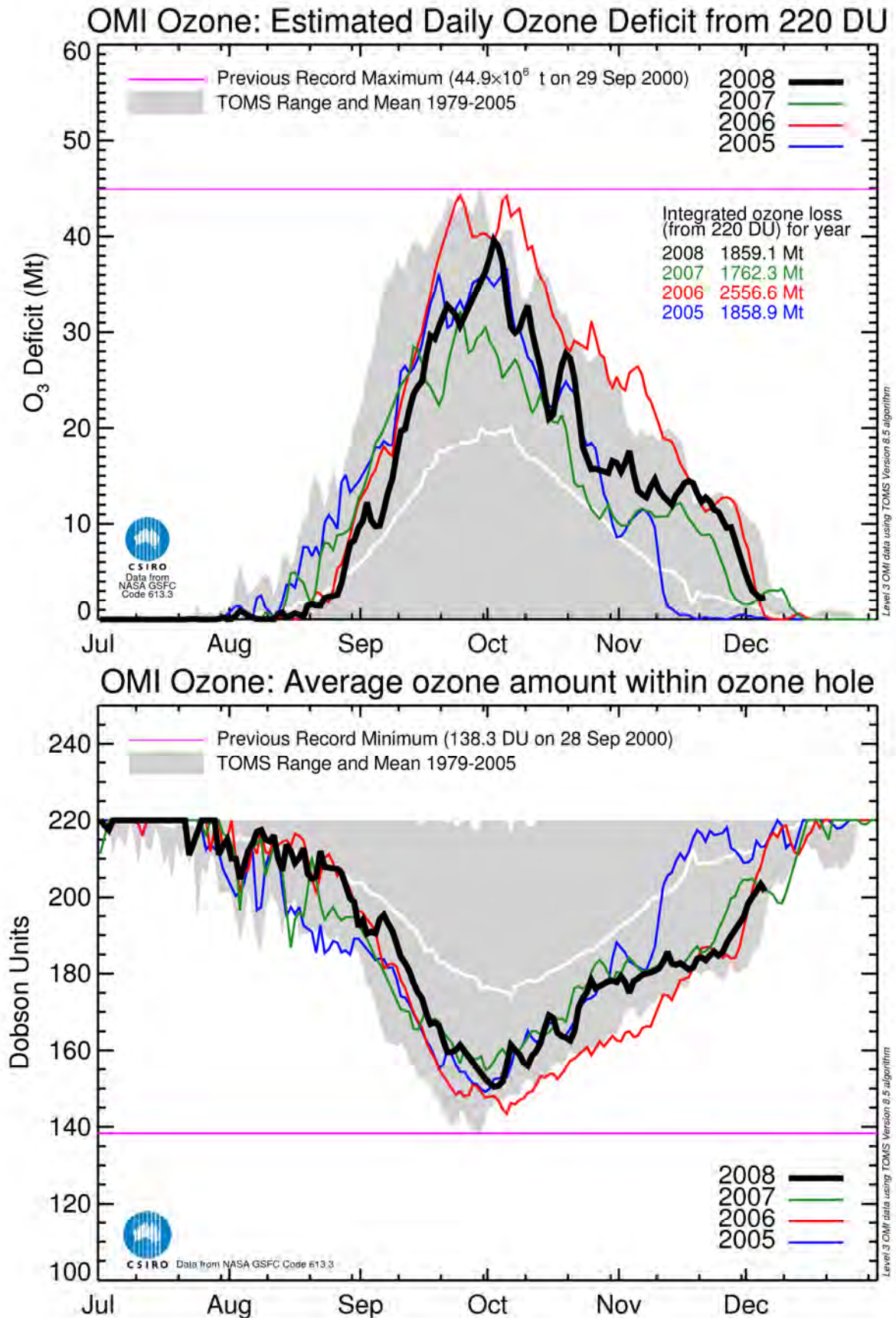
Figure 2: Estimated daily ozone deficit (top panel) and average ozone amount within the ozone hole (bottom panel) based on OMI satellite data, as of 5 December 2008.
