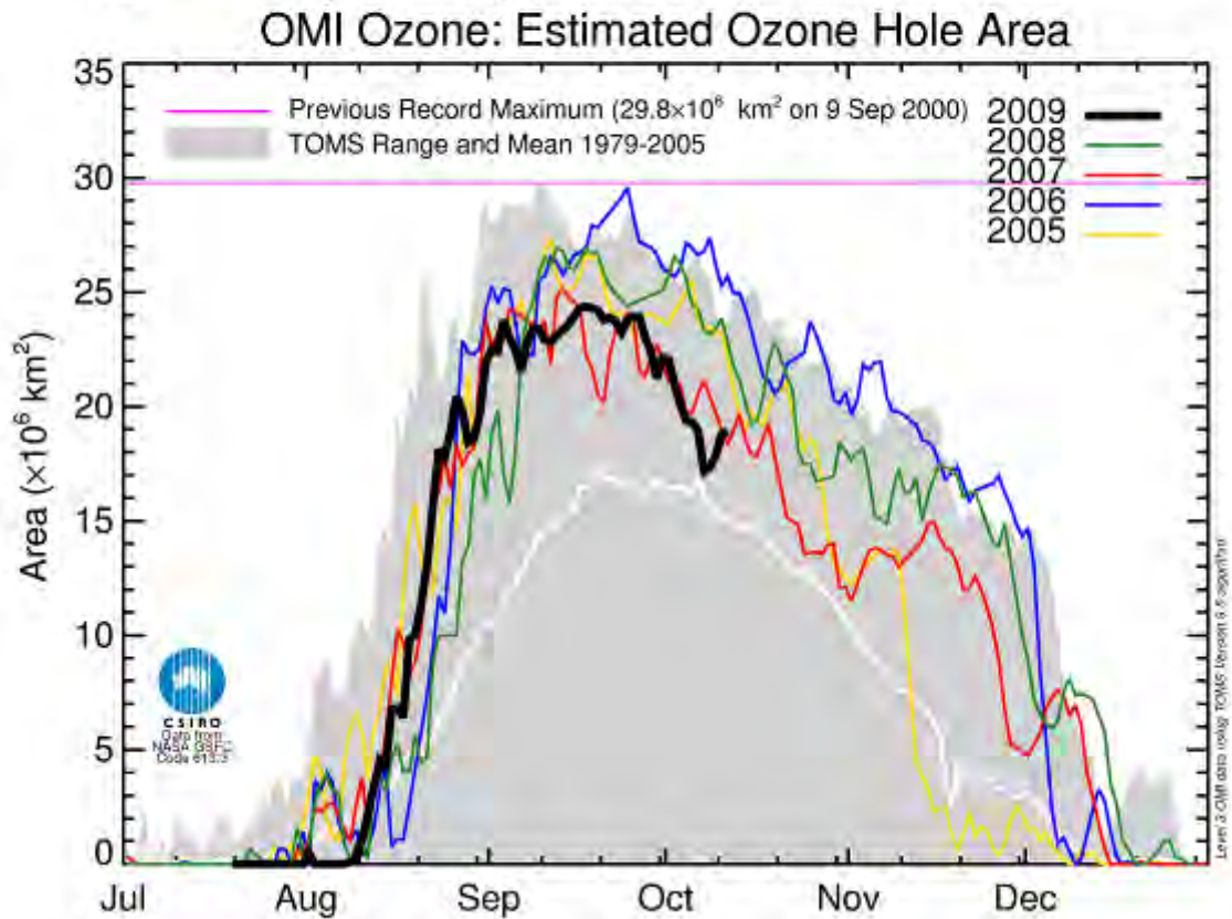
Figure 1: Ozone hole depth (top panel) and area (bottom panel) based on OMI satellite data, as of October 11, 2009.
