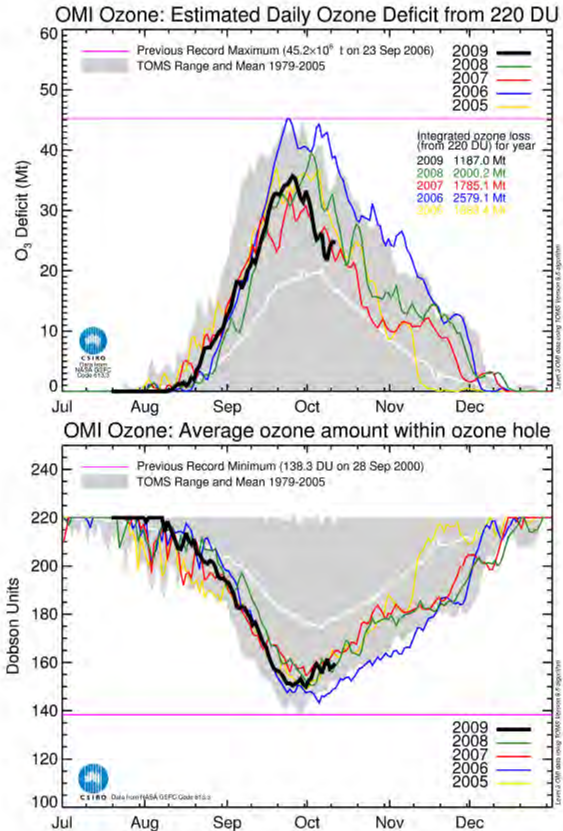
Figure 2: Estimated daily ozone deficit (top panel) and average ozone amount within the ozone hole (bottom panel) based on OMI satellite data, as of October 11, 2009.
