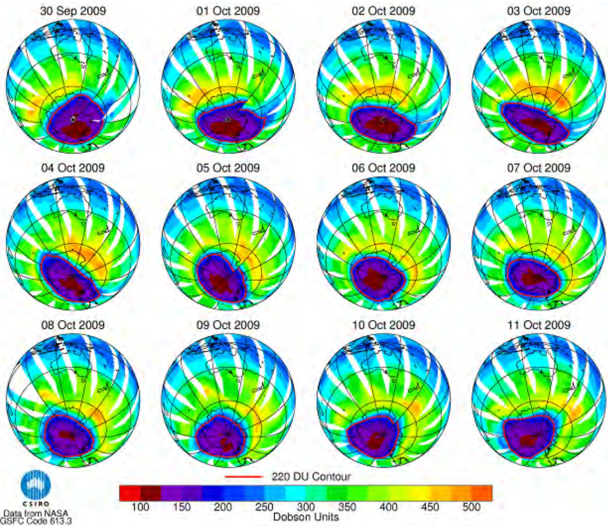
Figure 3: OMI ozone hole images for 30 September to 11 October 2009; the ozone hole boundary is indicated by the red 220 DU contour line. The white stripes are bad/missing data due to a physical obstruction in the OMI instrument field of view.
