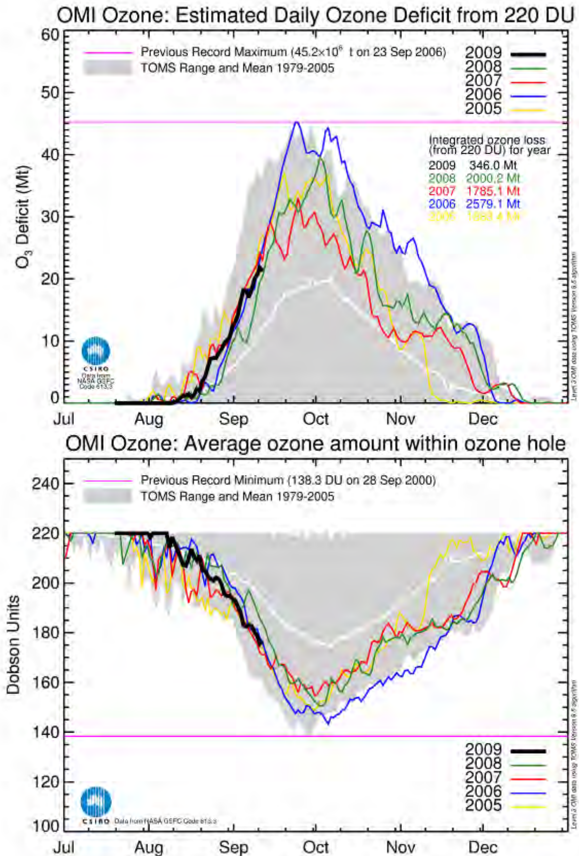
Figure 2: Estimated daily ozone deficit (top panel) and average ozone amount within the ozone hole (bottom panel) based on OMI satellite data, as of September 13, 2009.
