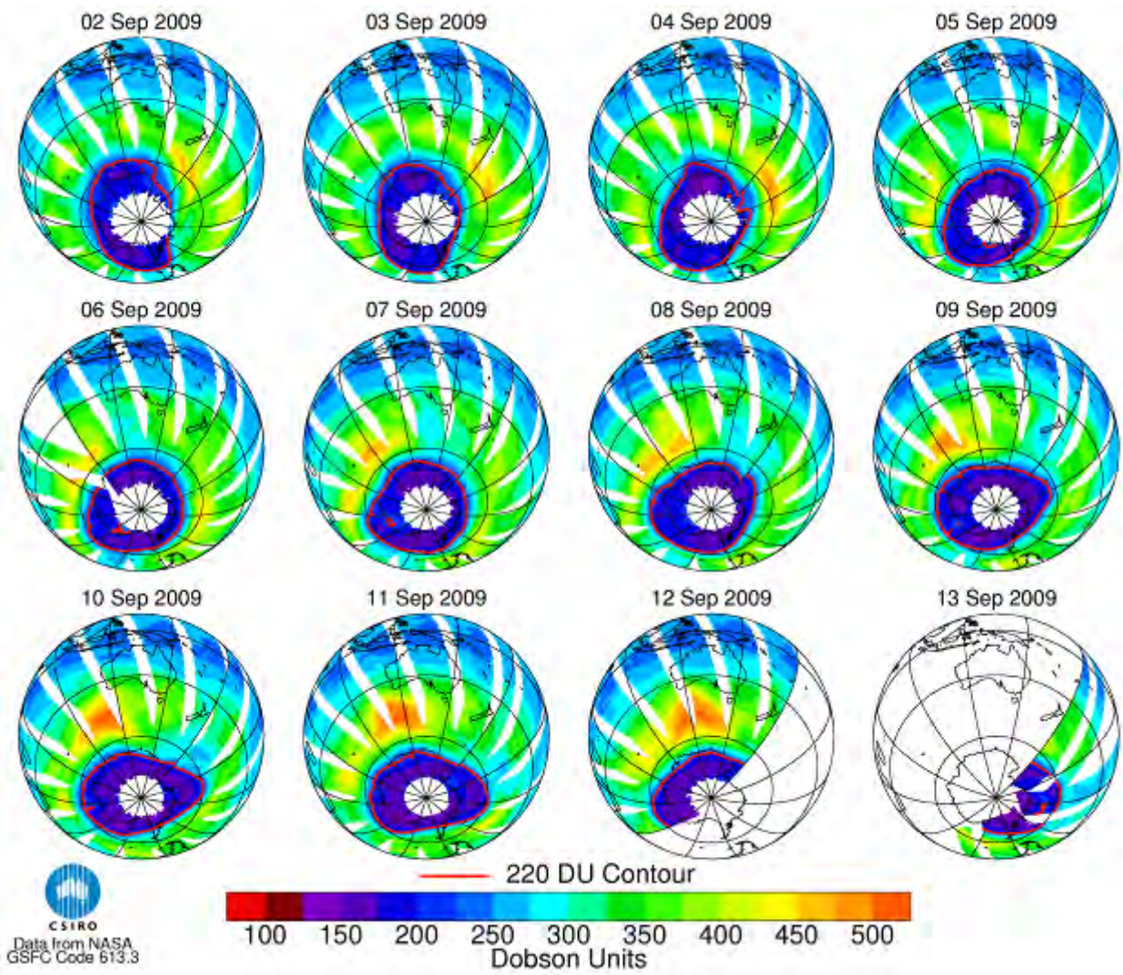
Figure 3: OMI ozone hole images for 2 to 13 September 2009; the ozone hole boundary is indicated by the red 220 DU contour line. The white area over Antarctica is missing data and indicates the approximate extent of the polar night. The OMI instrument requires solar radiation to the earth's surface in order to measure the column ozone abundance. The white stripes are bad/missing data due to a physical obstruction in the OMI instrument field of view.
