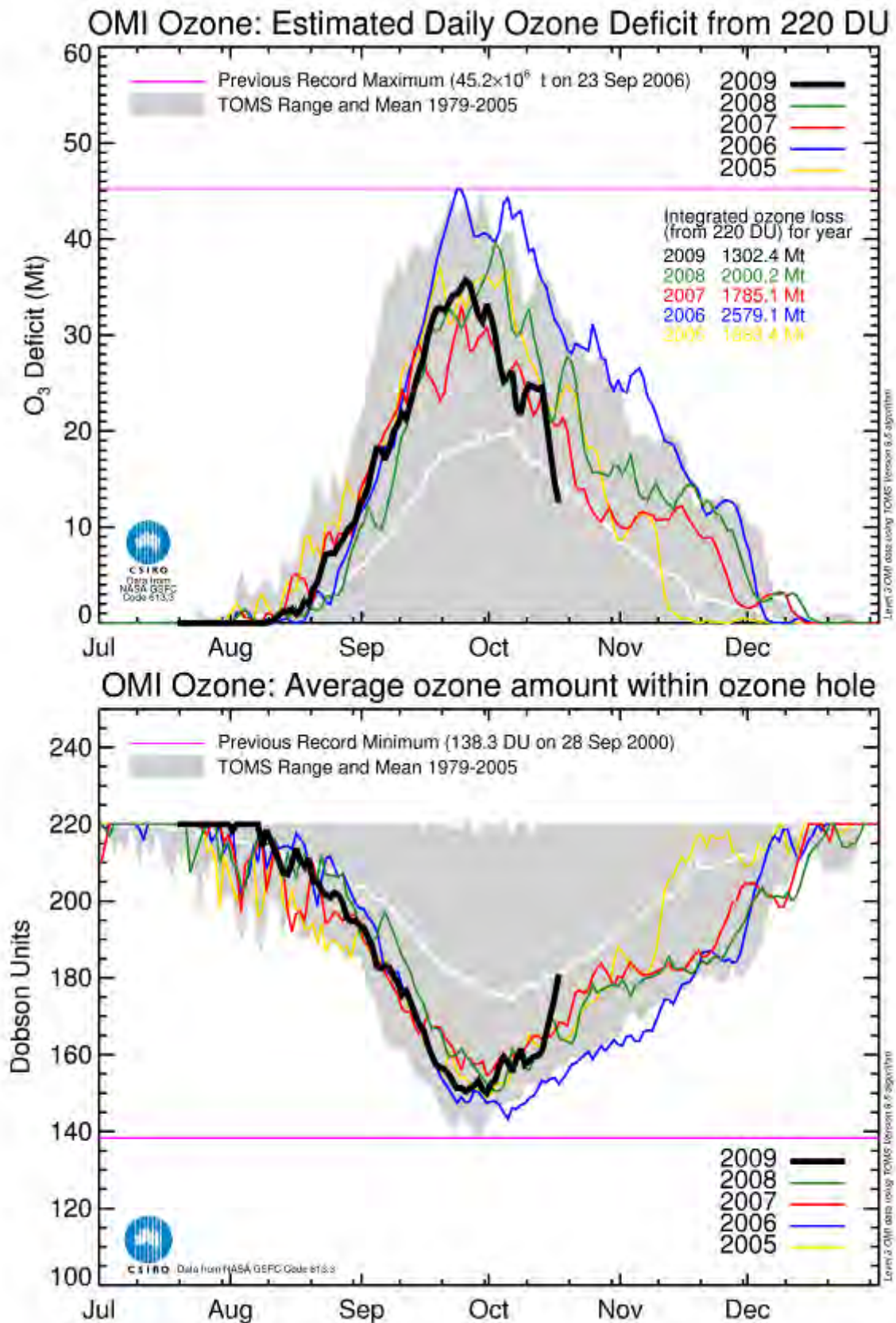
Figure 2: Estimated daily ozone deficit (top panel) and average ozone amount within the ozone hole (bottom panel) based on OMI satellite data, as of October 17, 2009.
