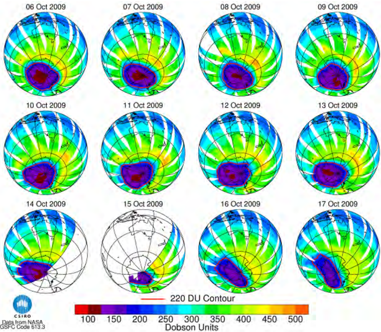
Figure 3: OMI ozone hole images for 6 to 17 October 2009; the ozone hole boundary is indicated by the red 220 DU contour line. The white stripes are bad/missing data due to a physical obstruction in the OMI instrument field of view.
