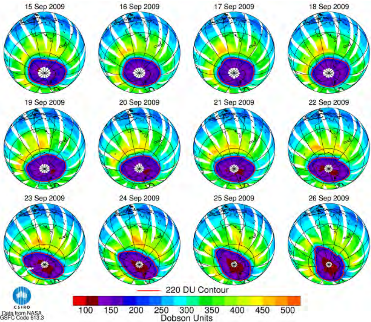
Figure 3: OMI ozone hole images for 15 to 26 September 2009; the ozone hole boundary is indicated by the red 220 DU contour line. The white area over Antarctica is missing data and indicates the approximate extent of the polar night. The OMI instrument requires solar radiation to the earth's surface in order to measure the column ozone abundance. The white stripes are bad/missing data due to a physical obstruction in the OMI instrument field of view.
