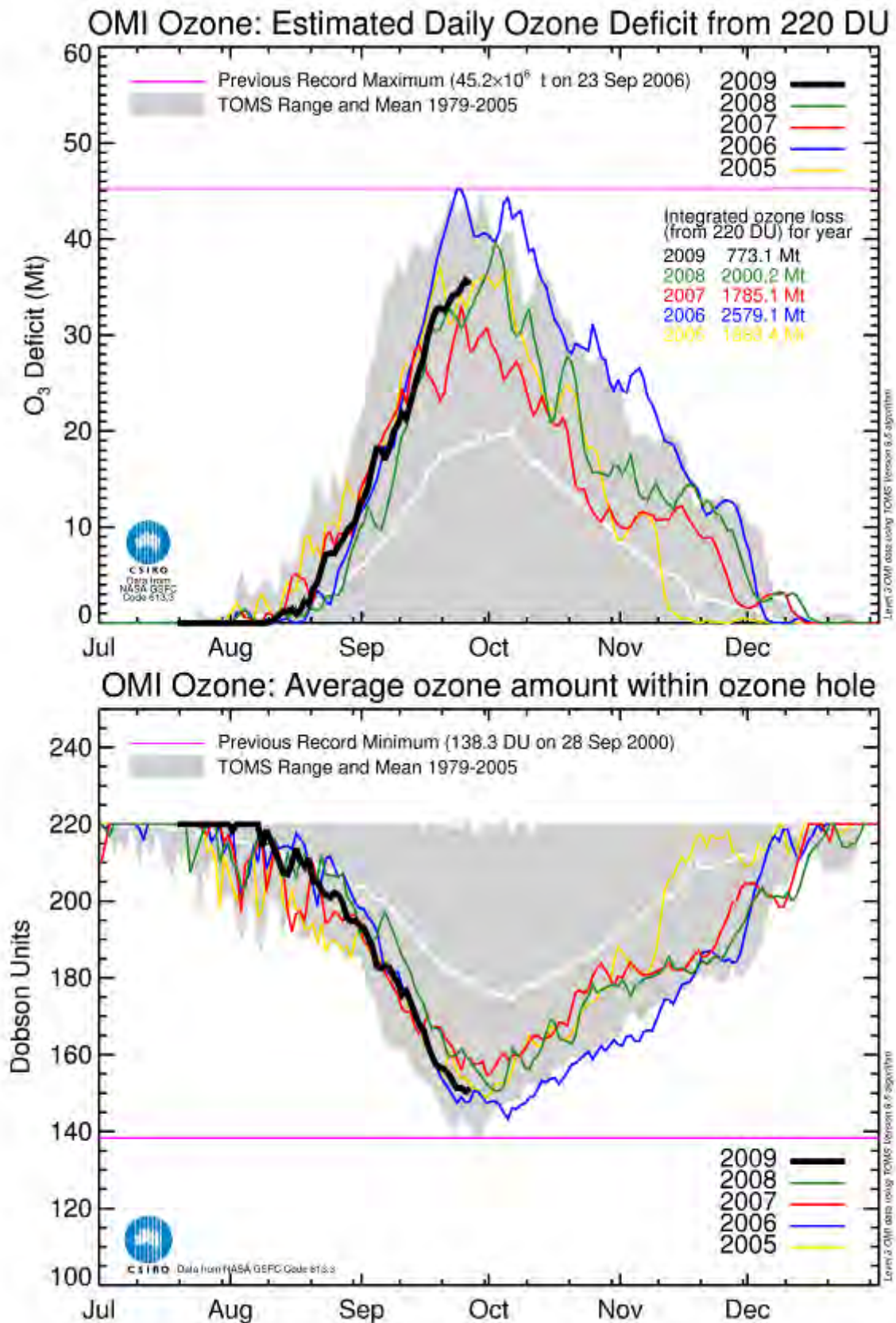
Figure 2: Estimated daily ozone deficit (top panel) and average ozone amount within the ozone hole (bottom panel) based on OMI satellite data, as of September 26, 2009.
