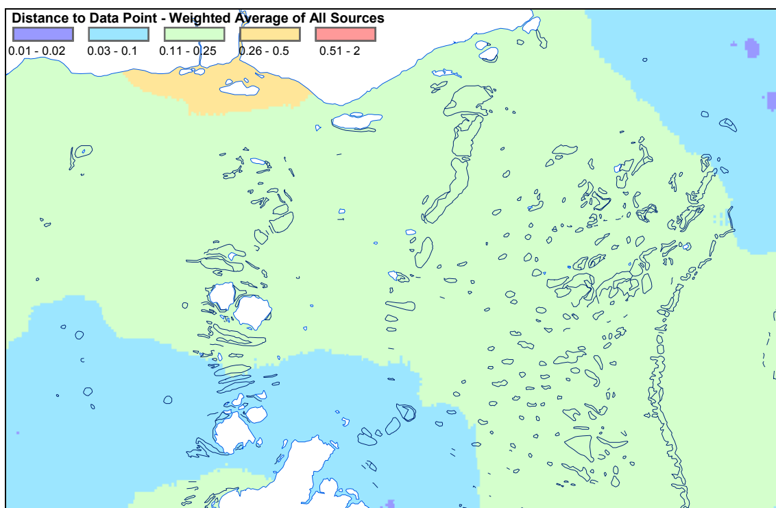
Figure 3.2-1 Map of overall gaps averaged across all seabed physical covariates, weighted by co-variate importance (section 2.8.1.2). That is, the distance-to-data of more the important co-variables has greater influence in the calculation of the average for each point.
