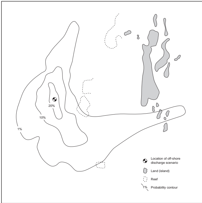
Figure 5. Conceptual result of a Monte Carlo exposure simulation.
