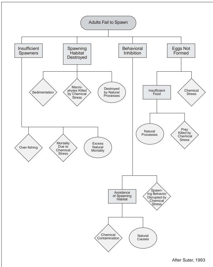
Figure 3. Event tree for the failure of adult fish to spawn.
