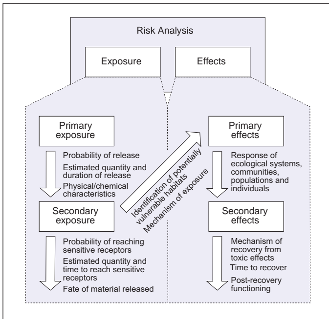
Figure 4. Steps in the ecological risk analysis methodology.
