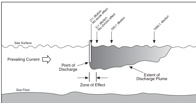
Figure 2. Conceptual representation of the zone of effect for an offshore discharge.
