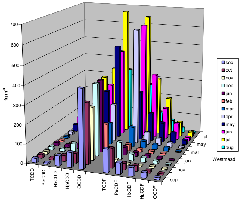
Figure 3.18 Westmead, NSW (residential area) homologue group profile.
