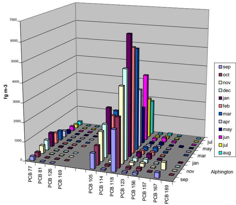
Figure 3.32 Alphington, Vic (residential) dioxin-like PCB congener profile.
