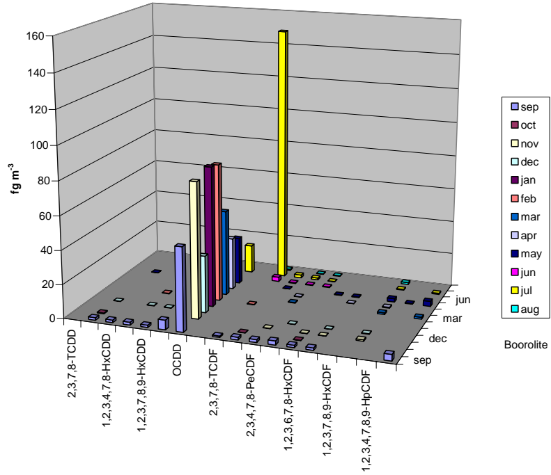
Figure 3.5 Boorolite, north-east Vic (rural) toxic congener profile.
