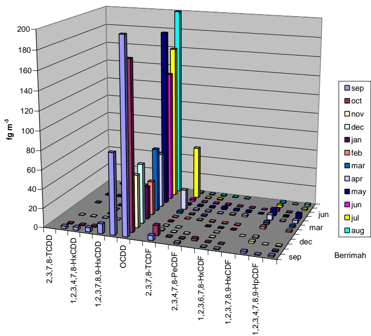
Figure 3.9 Berrimah, NT (remote - residential) toxic congener profile.
