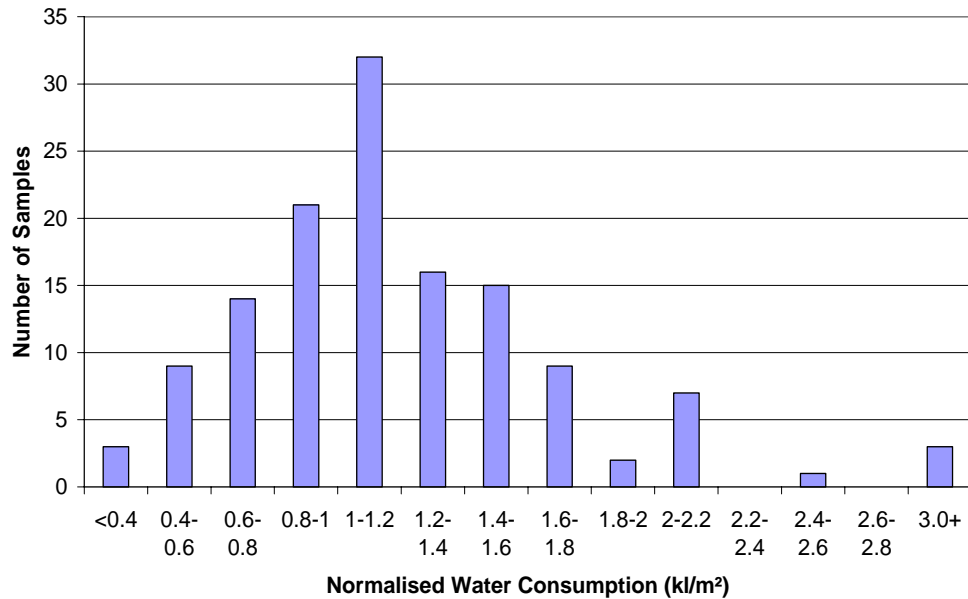
Figure 5. Distribution of office building water consumption after climate normalisation
