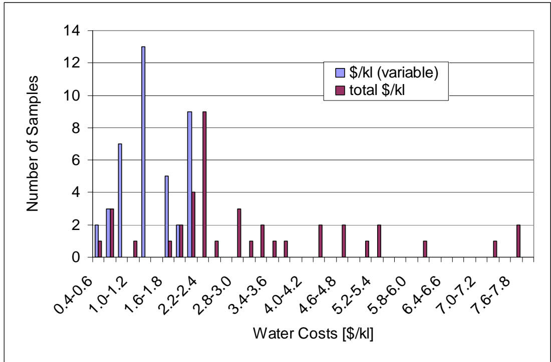
Figure 6. Distribution of the incremental and the total water costs; data points are for individual buildings within the sample for which bills were obtained.
