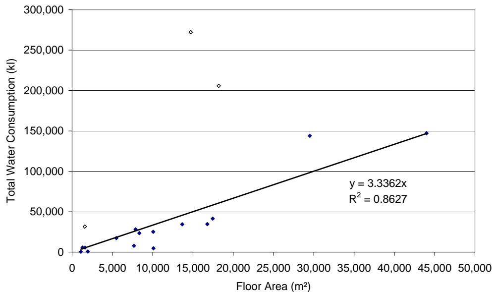
Figure 7. Water consumption – public office buildings. Hollow data points are outliers that have been excluded from the regression.
