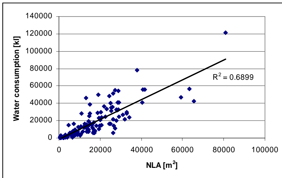
Figure 3. Water consumption as a function of floor area.
