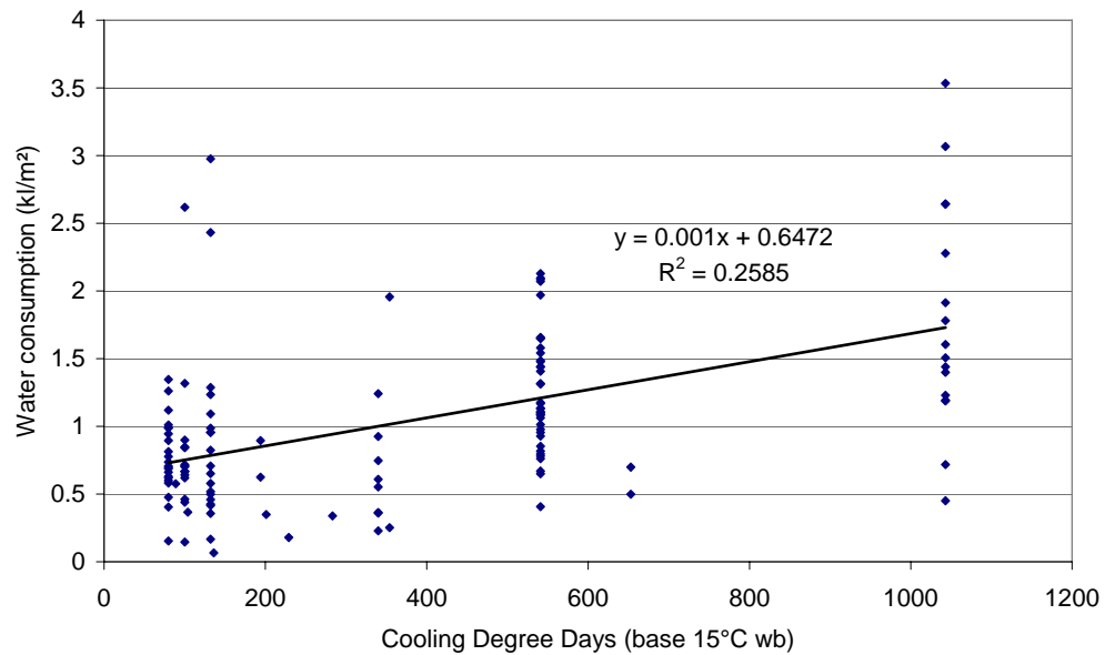
Figure 4. Water consumption versus cooling degree days.
