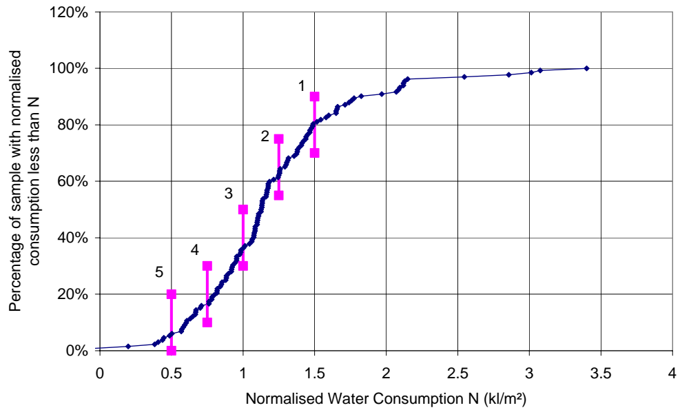
Figure 6. Cumulative frequency diagram for the sample population, showing proposed rating thresholds.
