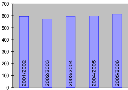
Law Courts (MJ/m²/annum)
