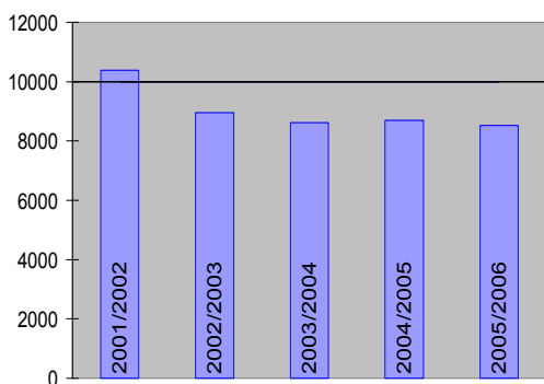
Office - Tenant Light and Power (MJ/person/annum) Target: 10 000 MJ/Person/Annum
