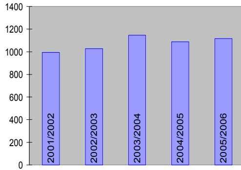
Laboratories (MJ/m²/annum)
