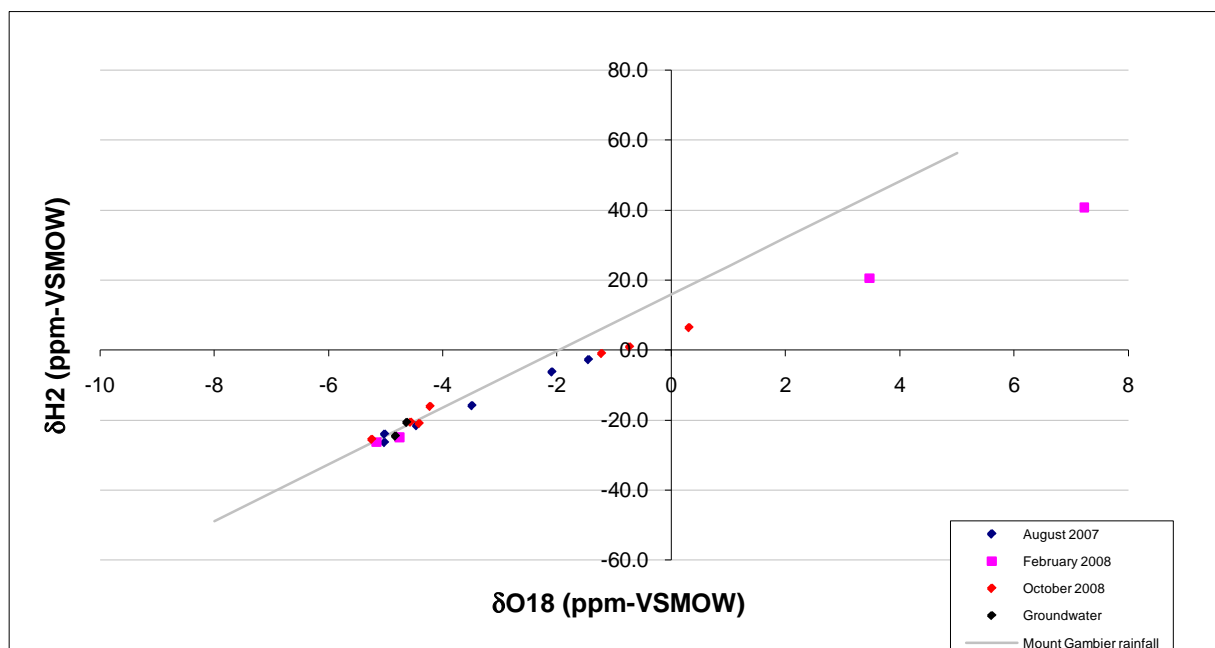
Figure 21. Stable isotope composition of surface water in Pick Swamp and Crescent Pond
