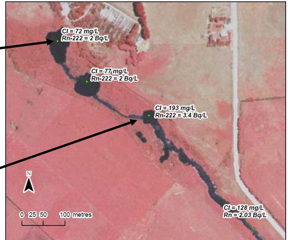
Figure 25. Chloride and radon-222 concentrations in Ewens Ponds (February 2008)
