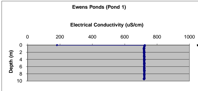
Figure 23. Sonde profile from Pond 1 of Ewens Ponds (February 2008)
