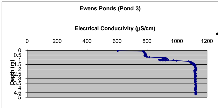
Figure 24. Sonde profile from Pond 3 of Ewens Ponds (February 2008)
