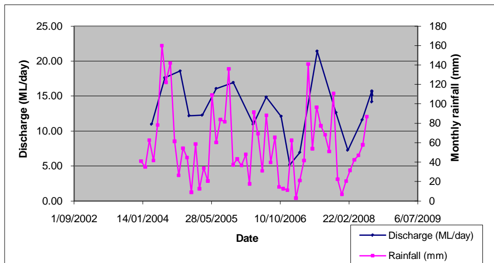
Figure 11. Cress Creek discharge and monthly rainfall measured at Mount Gambier
