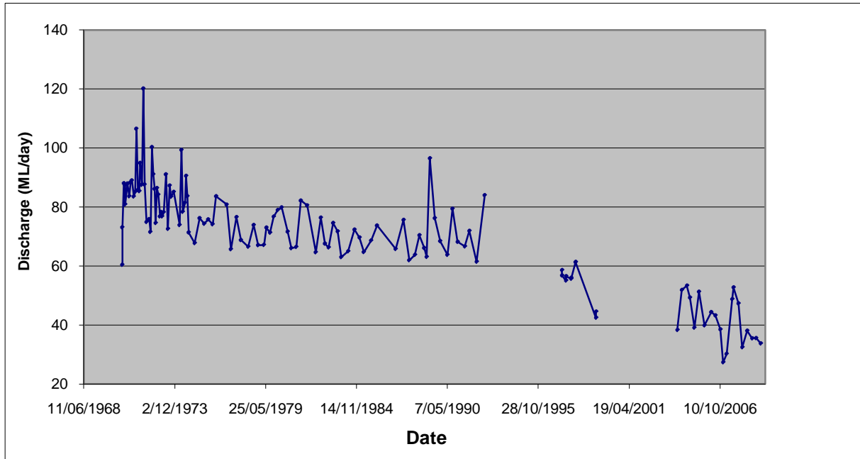
Figure 5. Piccaninnie Ponds discharge
