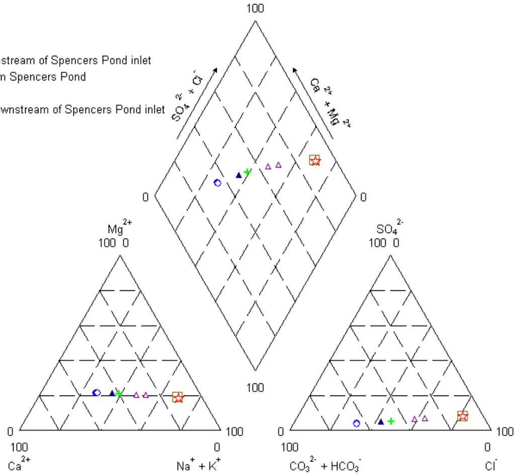
Figure 22. Piper plot of water chemistry in Ewens Ponds and Eight Mile Creek (locations shown on adjacent map)
