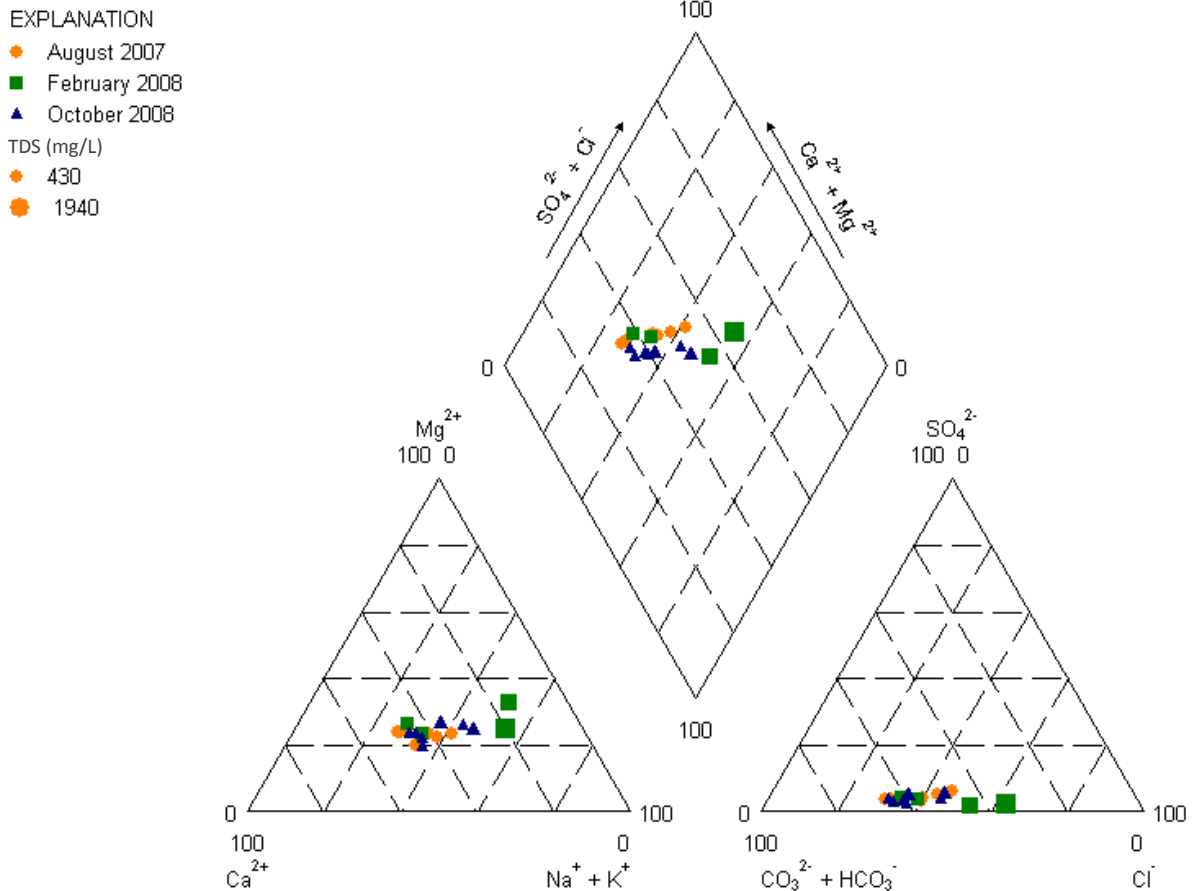
Figure 19. Piper plot of surface water chemistry at Pick Swamp and Crescent Pond
