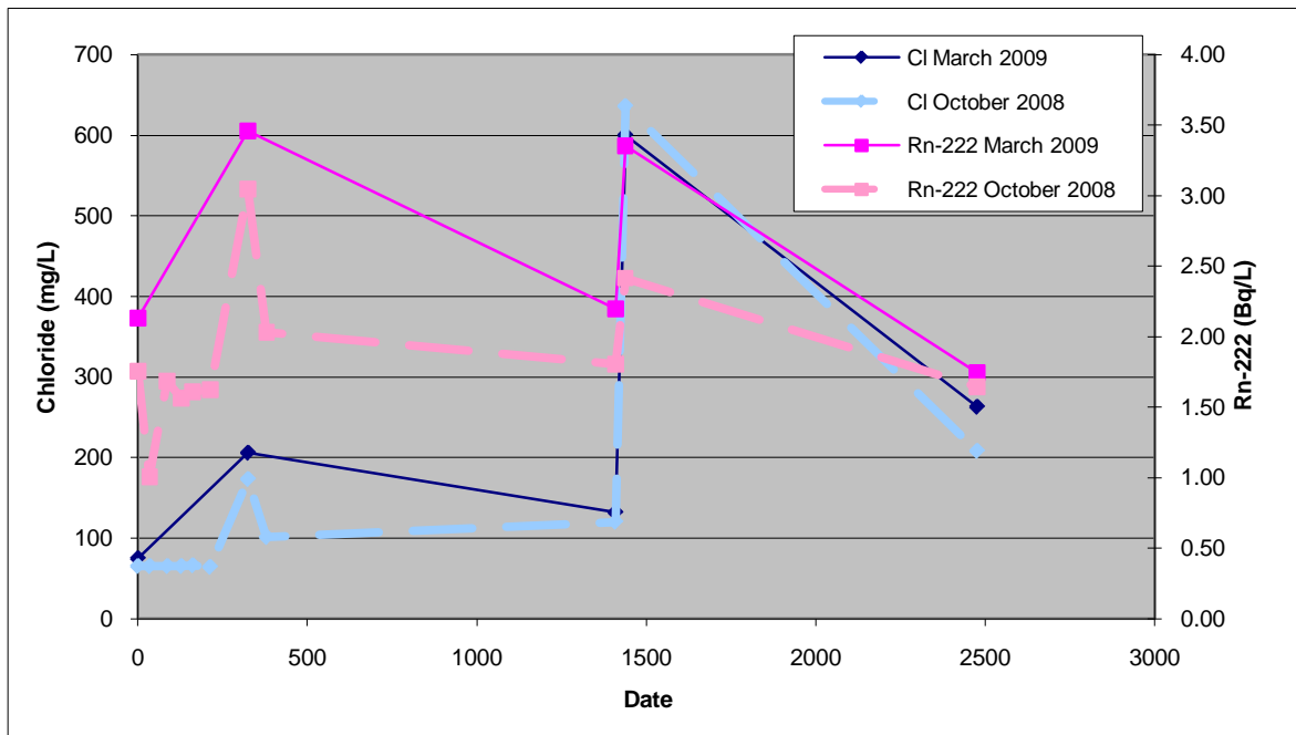
Figure 34. Comparison of March 2009 'monitoring strategy' results (solid lines) with October 2008 'detailed sampling' results (dashed line)
