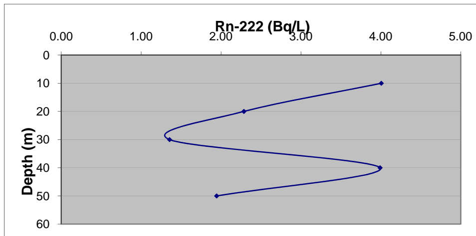
Figure 15. Radon-222 concentrations with depth in Piccaninnie Ponds
