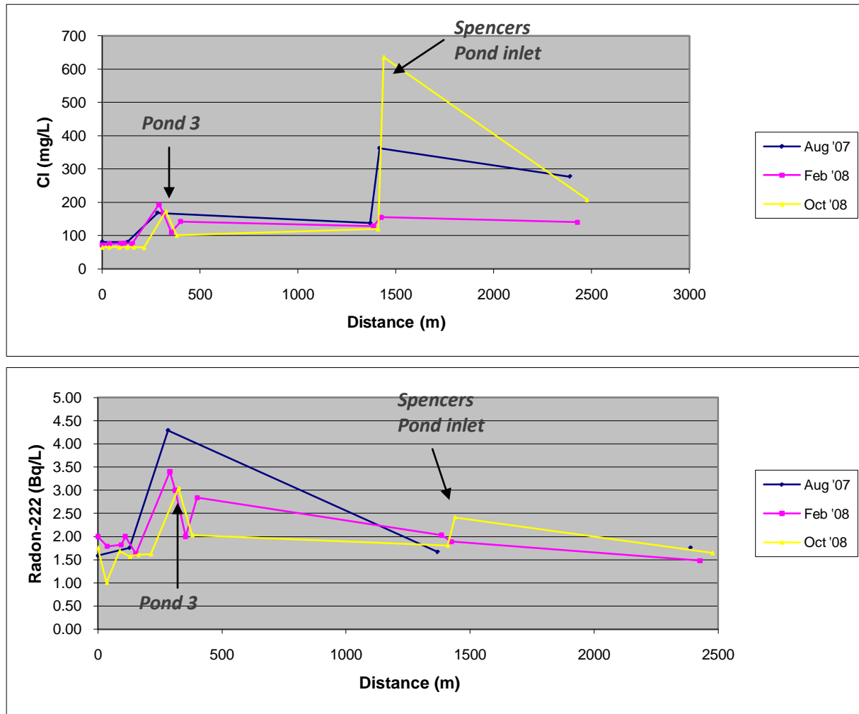
Figure 27. Seasonal variation in chloride and radon-222 concentrations with distance along Ewens Ponds and Eight Mile Creek
