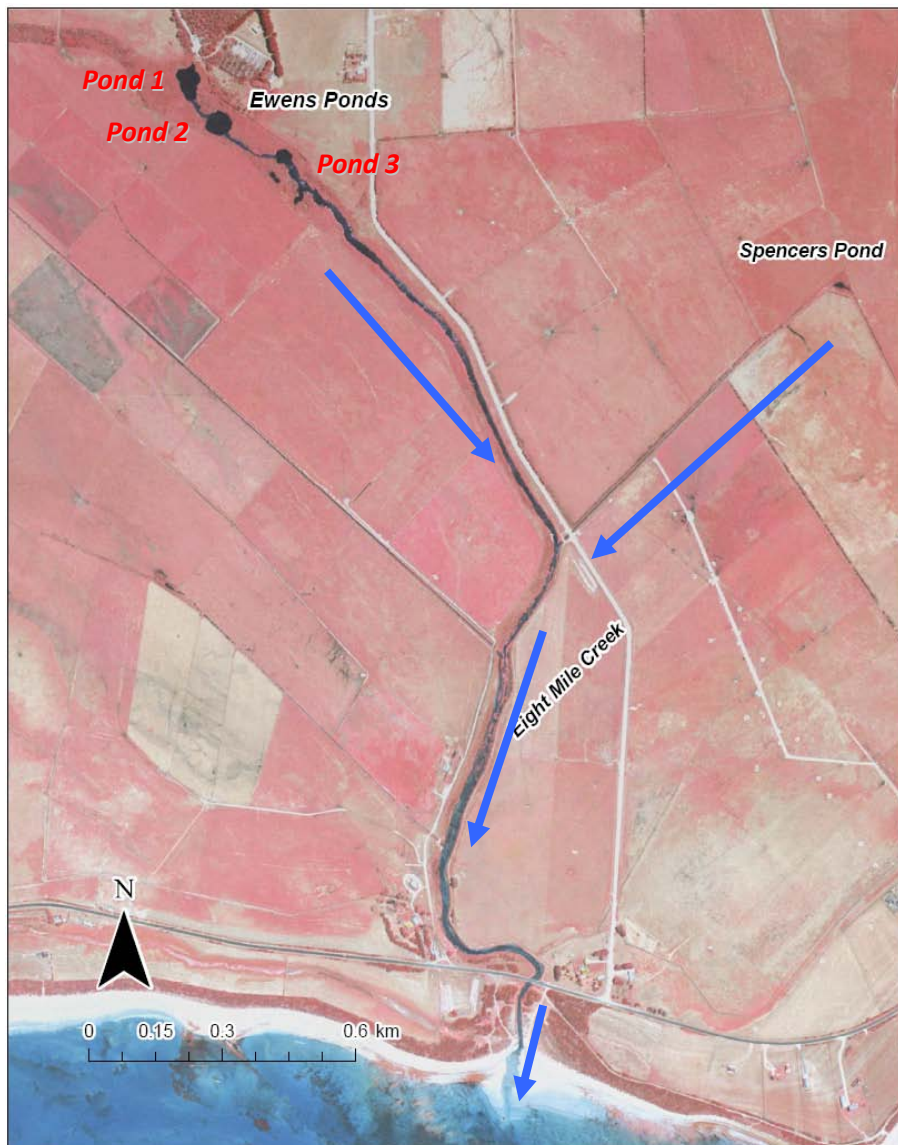
Figure 7. Ewens Ponds and Eight Mile Creek
