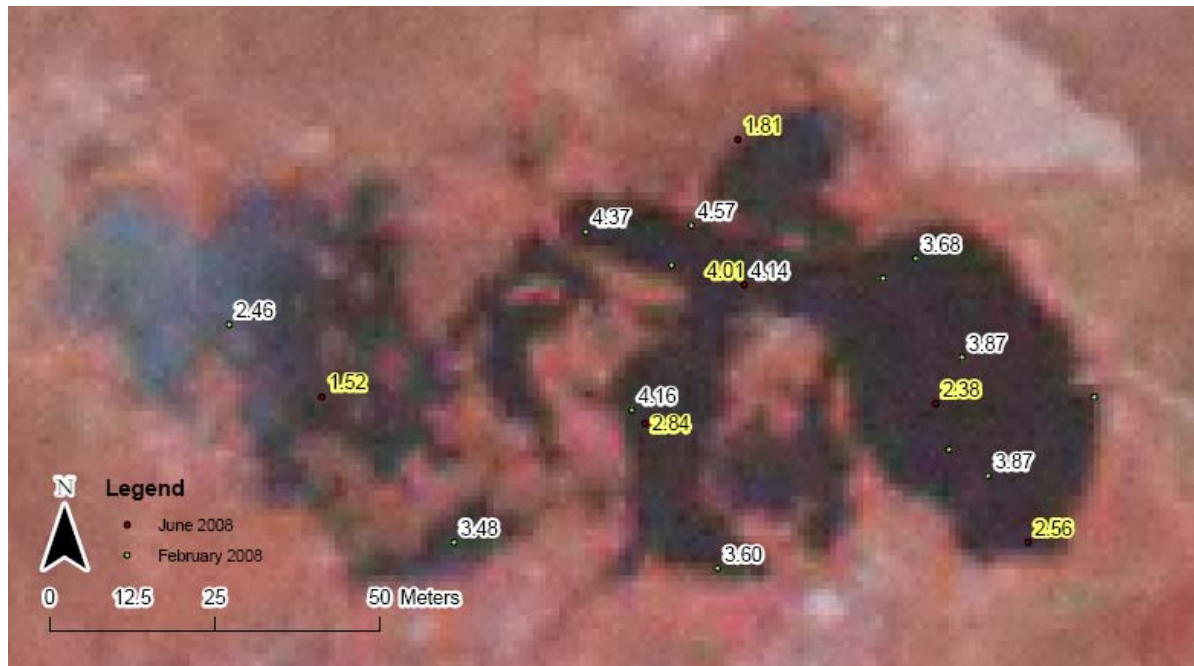
Figure 13. Radon-222 (Bq/L) in surface water at Piccaninnie Ponds, white halo indicates February 2008 sampling and yellow halo indicates June 2008 sampling
