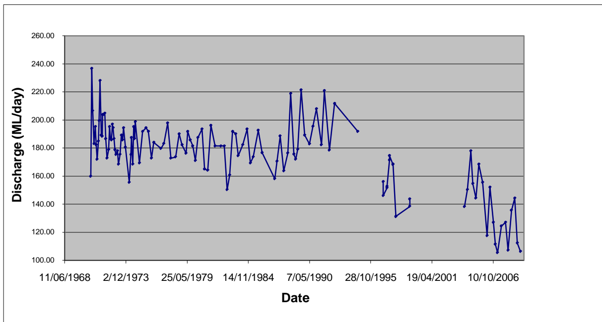
Figure 9. Eight Mile Creek discharge
