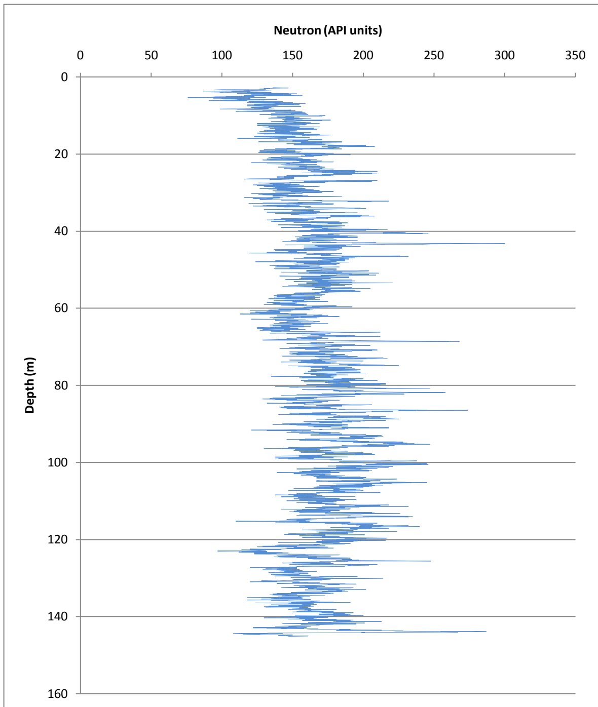
Figure 36. Neutron reading from geophysical log of Obswell CAR011
