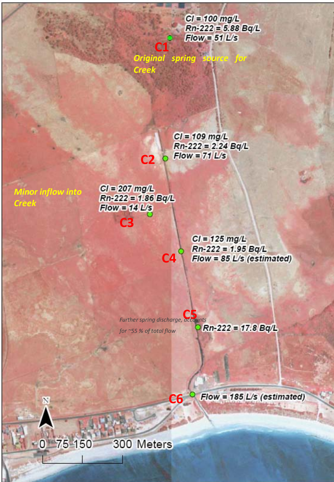
Figure 32. Conceptual model of flow and tracer concentrations (from August 2007 sampling) in Cress Creek
