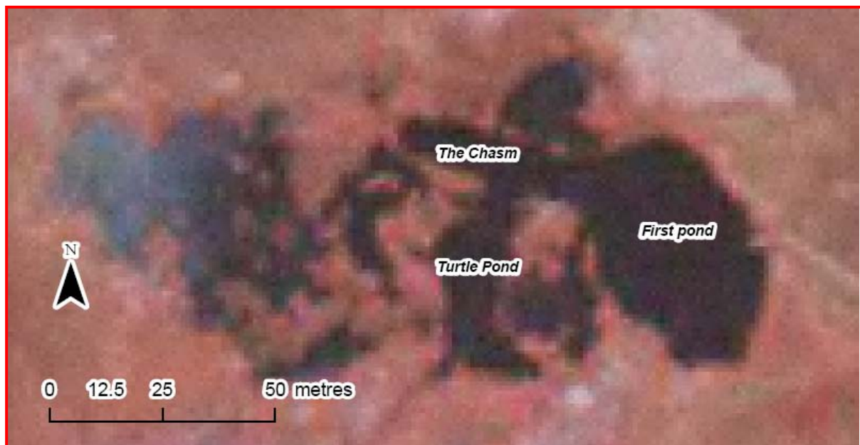
Figure 3. Piccaninnie Ponds and close-up of the Main Ponds
