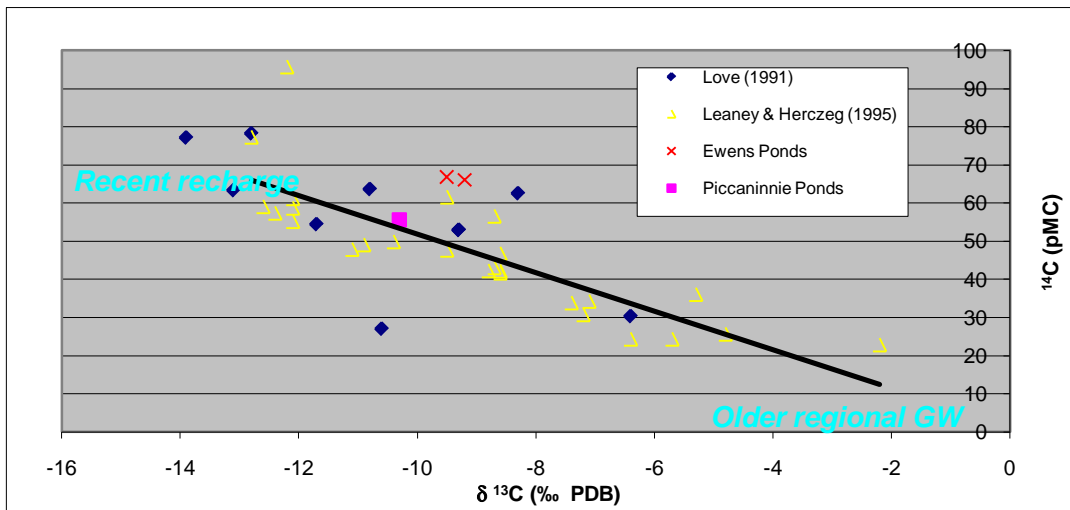
Figure 17. Carbon-14 isotope data from Piccaninnie Ponds and Ewens Ponds, compared with other regional TLA samples from previous studies (Leaney and Herczeg, 1995, and Love, 1991)
