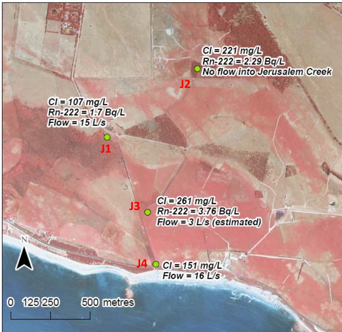
Figure 33. Conceptual model of flow and tracer concentrations (from August 2007 sampling) in Jerusalem Creek
